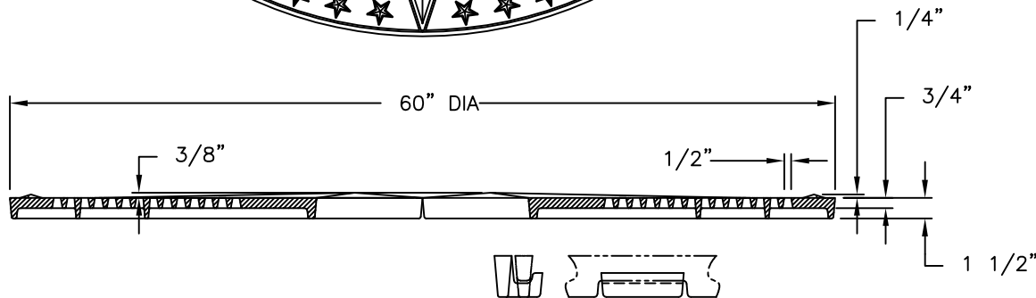
INTERLOCK ASSEMBLY DETAIL
